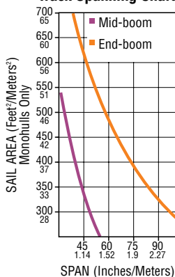
32 mm High-Beam Track Spanning Chart
