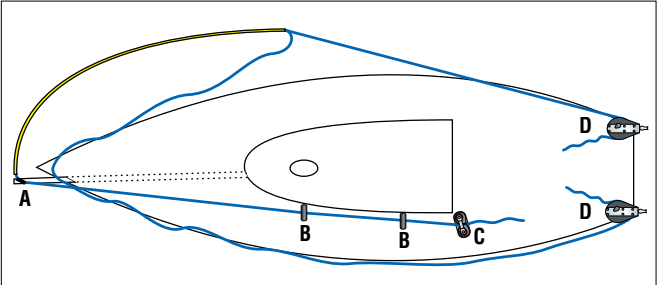
Asymmetrical on Sprit: Boats with asymmetrical spinnakers and retractable (or removable) bowsprits are rigged with a tack line leading through a block on the end of the sprit, and aft to a cleat or stopper. Two sheets attach to the clew of the sail, with the lazy sheet leading aft ahead of the headstay, over the sprit, and outside the shrouds and sheets.
