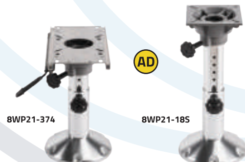
8WP21-374 ADJUSTABLE PEDESTAL W/ FORE & AFT SLIDE Features Adjusts from 12" to 18" Smooth, Thick Walled, Polished Anodized Aluminum 2 7/8" Diameter Pipe Locking Seat Mount w/ 360° Rotation 9" Diameter Base
