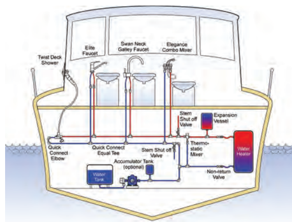
TYPICAL INSTALLATION
