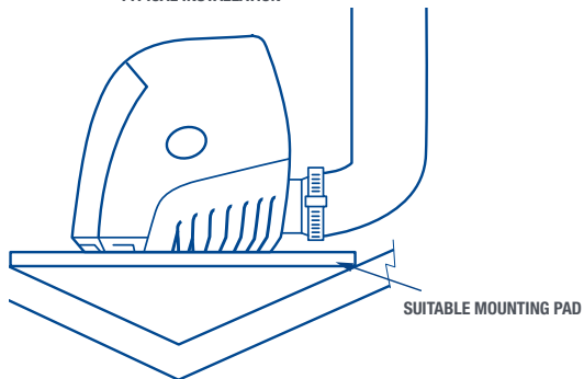
TYPICAL INSTALLATION
