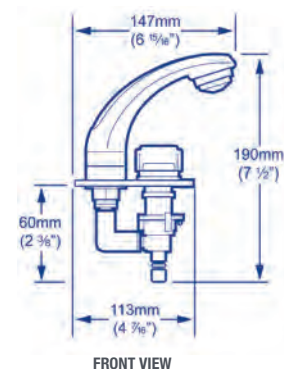
SINGLE FAUCET COLD ONLY
