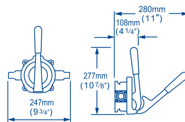
On Deck/Fixed Handle BP9005
