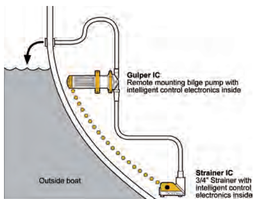
TYPICAL INSTALLATION
