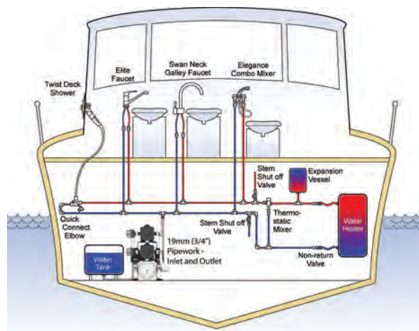
TYPICAL INSTALLATION
