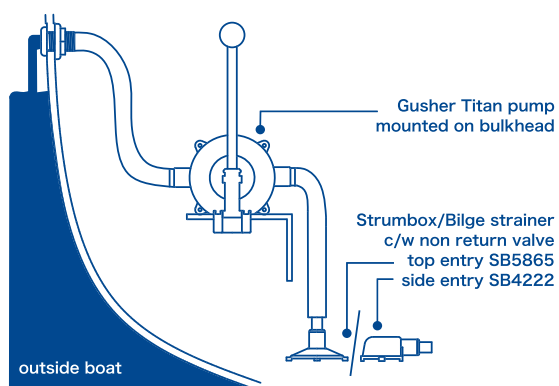
TYPICAL INSTALLATION
