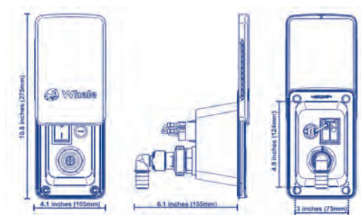
4 IN 1 FITTING
