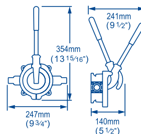
Bulkhead/Removable Handle BP9021
