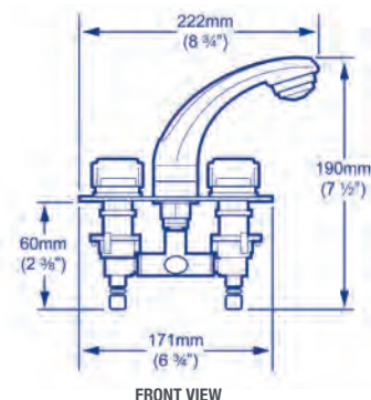
MIXER FAUCET STANDARD OUTLET
