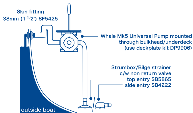
TYPICAL INSTALLATION
