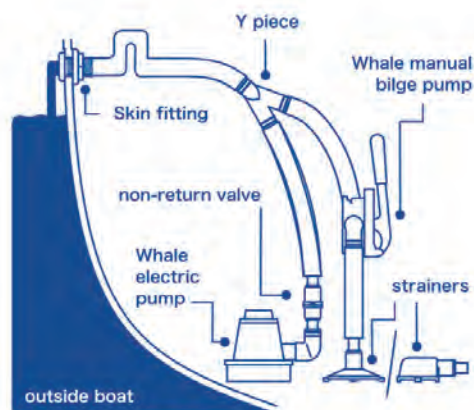
TYPICAL INSTALLATION
