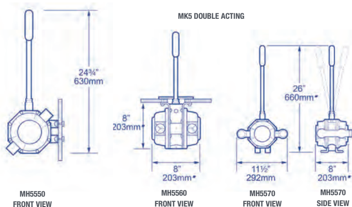
MK5 DOUBLE ACTING MANUAL BILGE PUMP
