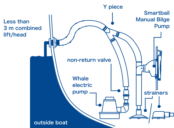
TYPICAL INSTALLATION
