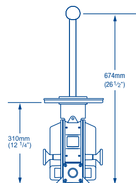
BP3020 SIDE VIEW
