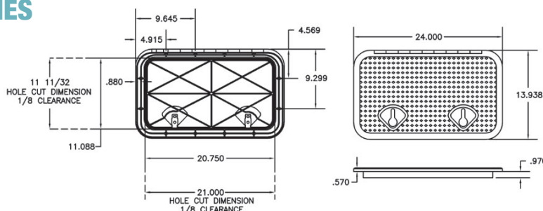
HT1424
