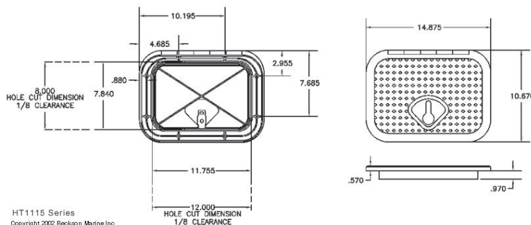
HT1115
