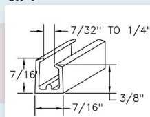
CH-1
